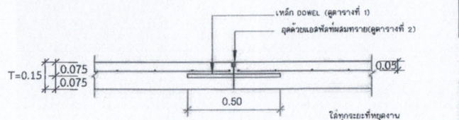
CONSTRUCTION JOINT
