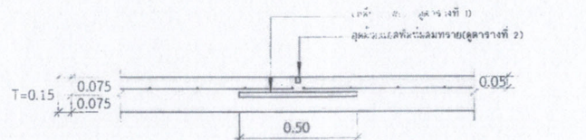
CONTRACTION JOINT
